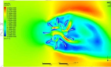
CFD analysis of a VAWT
